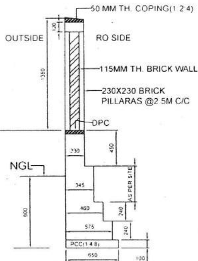
SECTION OF COMPOUND WALL (FILLING UP TO 600MM)
