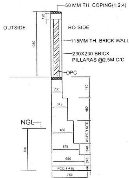
SECTION OF COMPOUND WALL (FILLING UPTO 1200MM)
