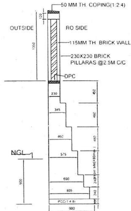
SECTION OF COMPOUND WALL (FILLING UPTO 1800MM)
