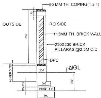
SECTION OF COMPOUND WALL WITHOUT ANY FILLING
